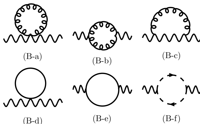
Figure 8: Diagrams for the one-loop self energy of A_0 . The curly line represents the propagator of A_i . The solid line represents the propagator of X_{AB} . The dashed line represents the propagator of \psi^A .
