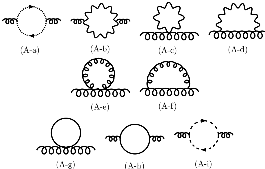
Figure 7: Diagrams for the one-loop self energy of A_i . The curly line represents the propagator of A_i . The wavy line represents the propagator of A_0 . The dotted line represents the propagator of the ghost. The solid line represents the propagator of X_{AB} . The dashed line represents the propagator of \psi^A .
