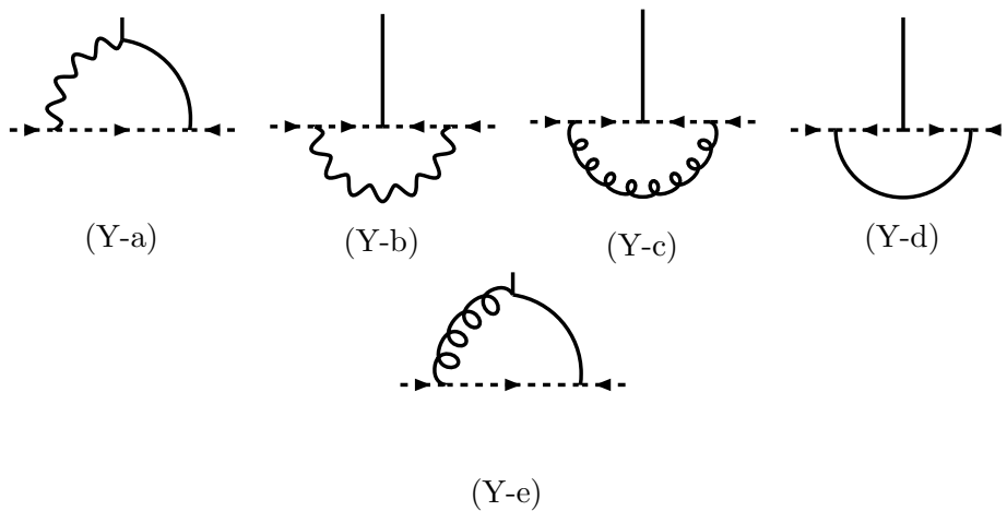
Figure 12: Diagrams for the one-loop correction to the Yukawa interaction. The curly line represents the propagator of A_i . The wavy line represents the propagator of A_0 . The solid line represents the propagator of X_{AB} . The dashed line represents the propagator of \psi^A .
