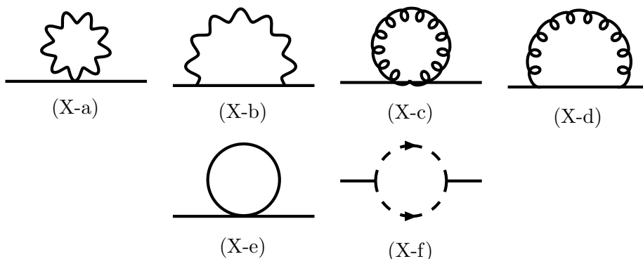
Figure 2: Diagrams for the one-loop self-energy of X_{AB} . The curly line represents the propagator of A_i . The wavy line represents the propagator of A_0 . The solid line represents the propagator of X_{AB} . The dashed line represents the propagator of \psi^A .
