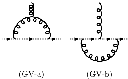
Figure 11: Diagrams for the one-loop correction to the ghost-ghost-gauge interaction vertex. The curly line represents the propagator of A_i . The dotted line represents the propagator of the ghost.
